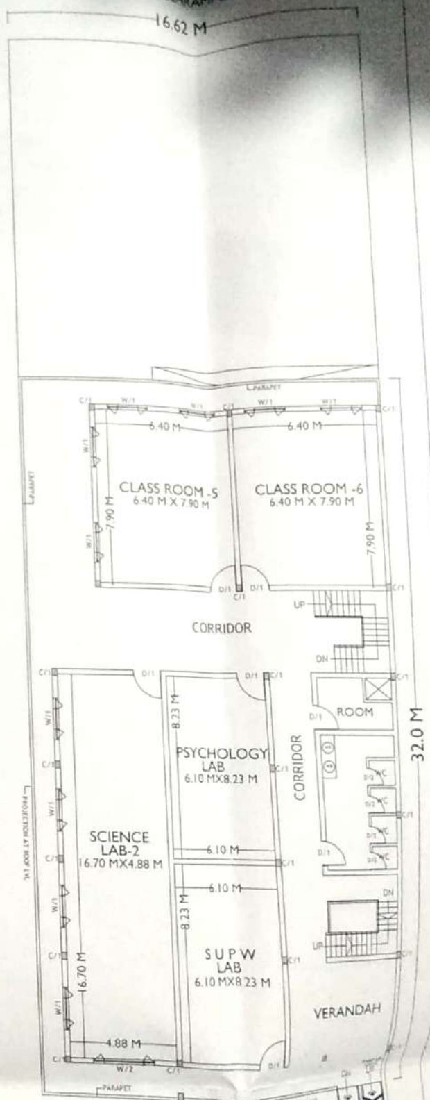
← SECOND FLOOR PLAN S.F COV. - 531.84 SQM
