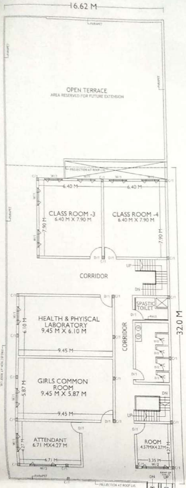
← FIRST FLOOR PLAN F.F COV. - 531.84 SQM
